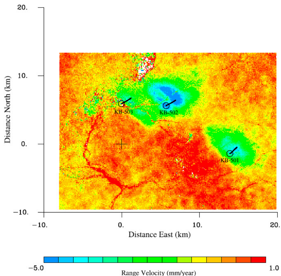
Fig. 1: InSAR displacement measured towards the satellite in mm/year for the In Salah field in Algeria, from year 2003 to year 2007. The three CO 2 injection wells are labelled (KB-501,
